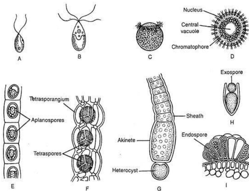
Fig. 3.17: Asexual spores in algae : A. Biflagellate microzoospore, and B. Quadriflagellate microzoospore of Ulothrix sp., C. Multiflagellate zoospore of Oedogonium sp., D. Synzoospore of Vaucheria sp., E. Aplanospores of Ulothrix sp., F. Tetraspores of Polysiphonia sp., G. Akinete of Gloeotrichia sp., H. Exospore of Chamaesiphon incrustans , and I. Endospores of Dermocarpa prasina
