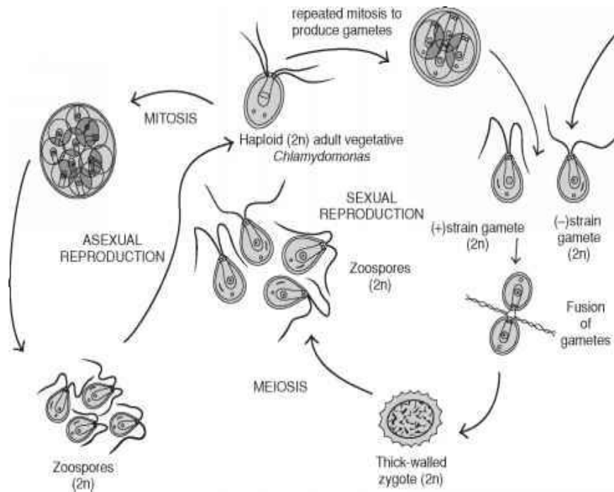
Zoospores of chlamydomonas
